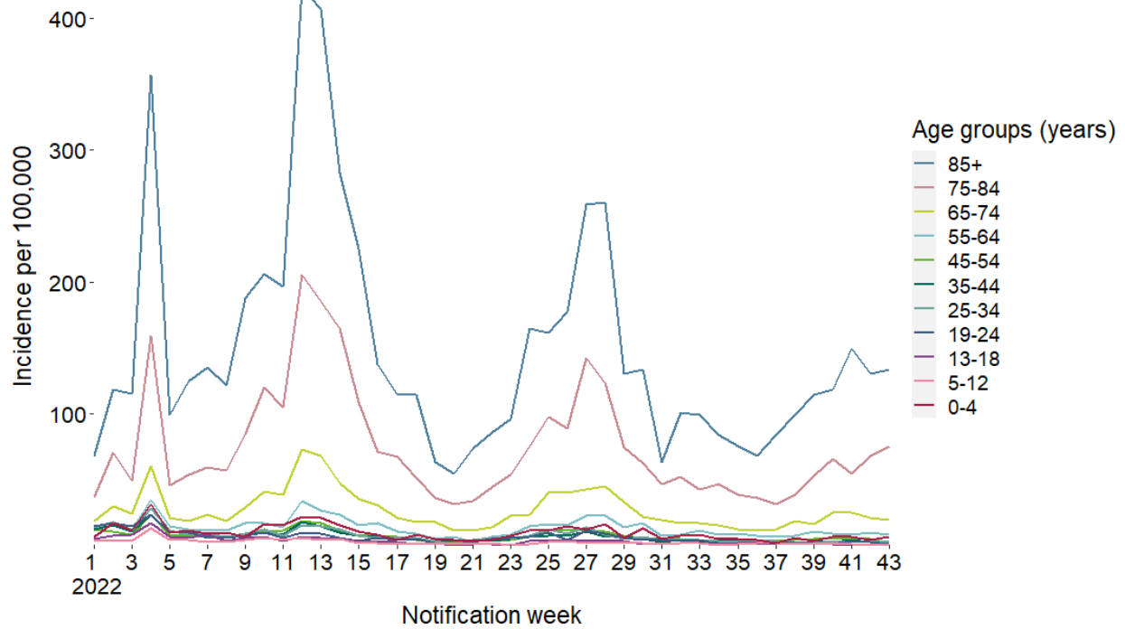
Figure 7: Incidence rate by age group of hospitalisations among confirmed COVID-19 cases on CIDR in Ireland between week 1, 2022 and week 43, 2022
