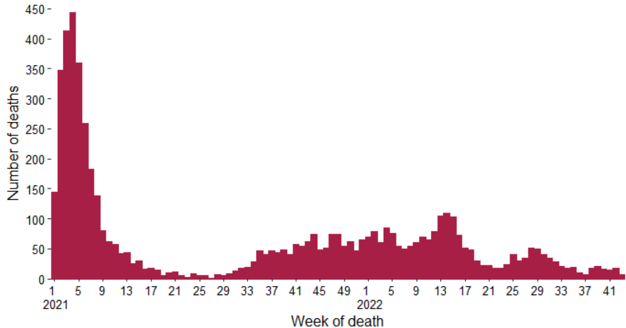
Figure 10: Total number of COVID-19 deaths notified by week of death, cases with a date of notification from week 1, 2021 to 43, 2022. Date of death missing for 0 of the reported deaths
