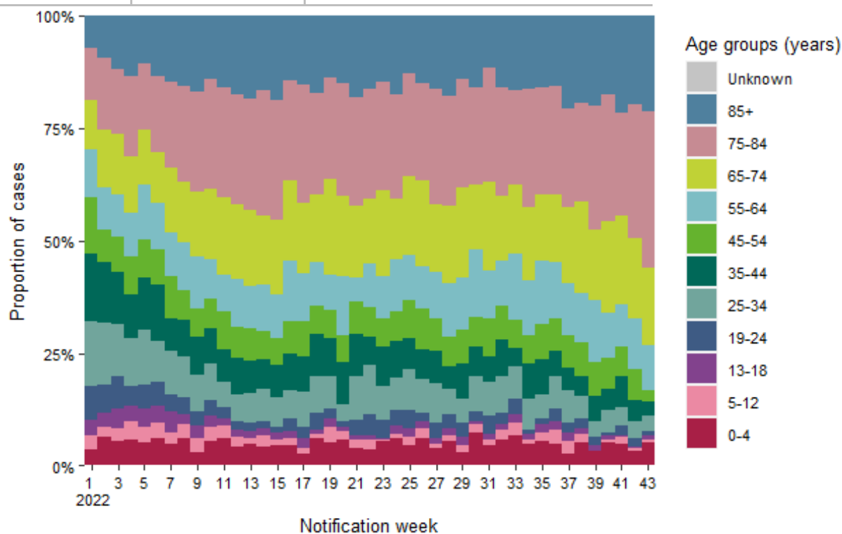
Figure 6: Age distribution of hospitalised confirmed COVID-19 cases notified on CIDR in Ireland between week 1, 2022 and week 43, 2022
