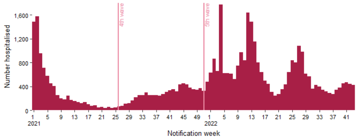
Figure 5: Hospitalisations among confirmed COVID-19 cases notified on CIDR in Ireland between week 1, 2021 and week 43, 2022
