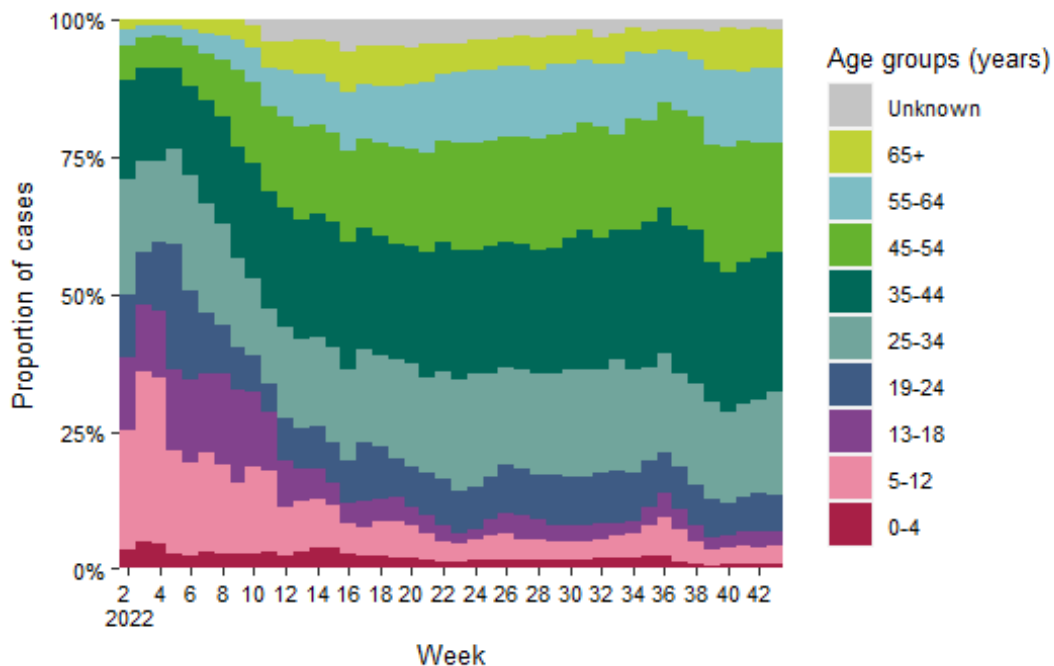
Figure 14: Age distribution of COVID-19 cases who registered a positive antigen test on the HSE Positive Antigen Portal by week of registration 11 in Ireland between week 2 8 , 2022 and week 43, 2022
