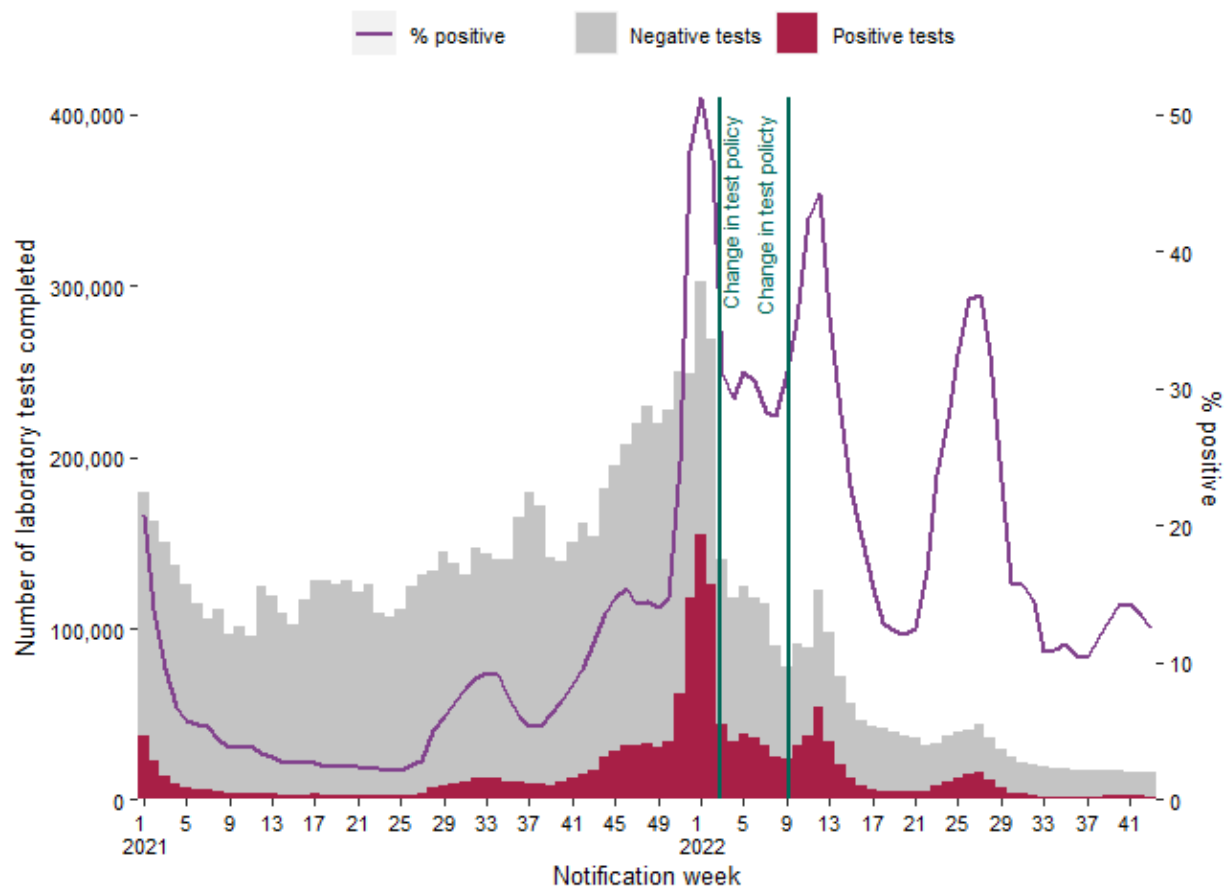
Figure 12: Number of completed laboratory tests by result and % positive tests 6 in Ireland between week 1, 2021 and week 43, 2022. Data source: Deloitte Ireland LLP 7, 8
