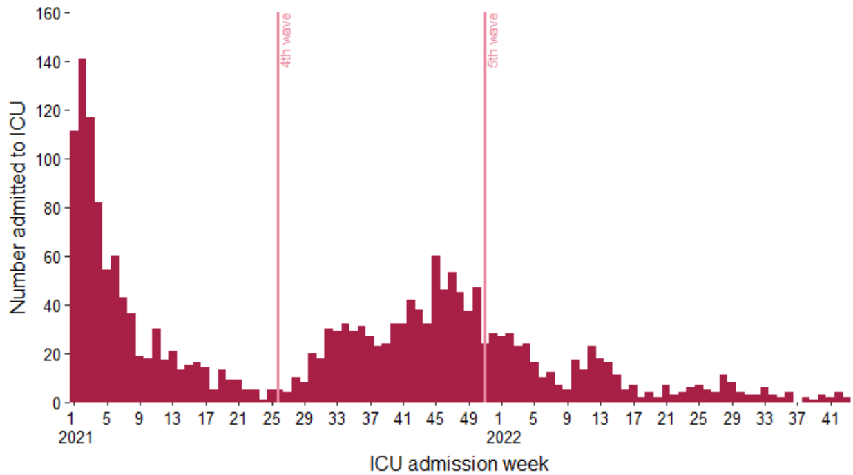
Figure 8: Number of ICU COVID-19 ICU admissions in Ireland by week of ICU admission, between week 1, 2021 and week 43, 2022 5
