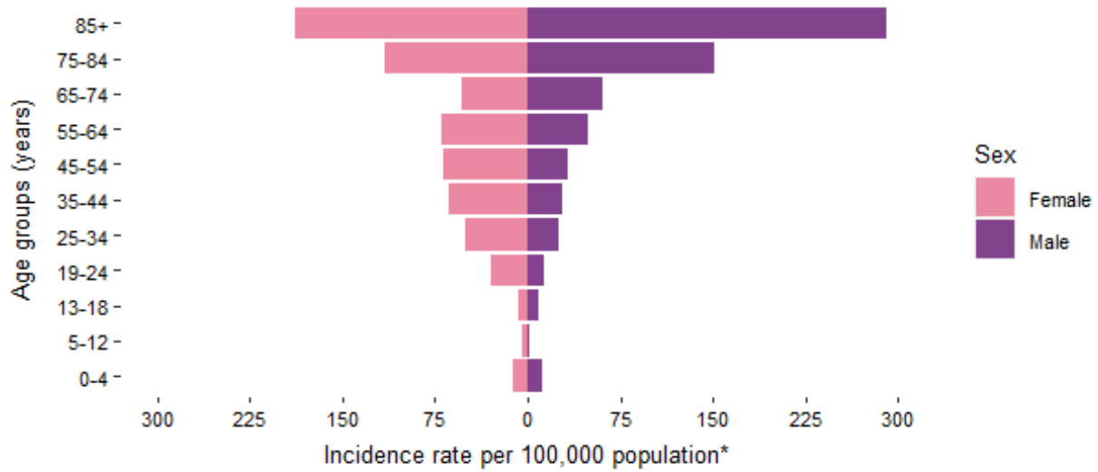
Figure 2: Cumulative age and sex specific incidence rates of confirmed COVID-19 cases per 100,000 population for current week 43, 2022
