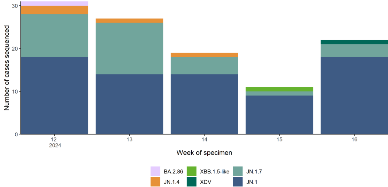
Figure 4a: SARS-CoV-2 whole genome sequencing results by week specimen collected from week 12 2024 to week 16 2024, Ireland. 2
