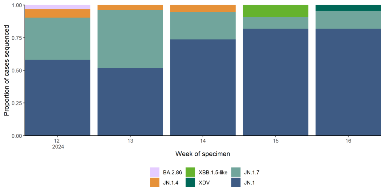
Figure 4b: SARS-CoV-2 whole genome sequencing results by proportion by week specimen collected from week 12 2024 to week 16 2024, Ireland.
