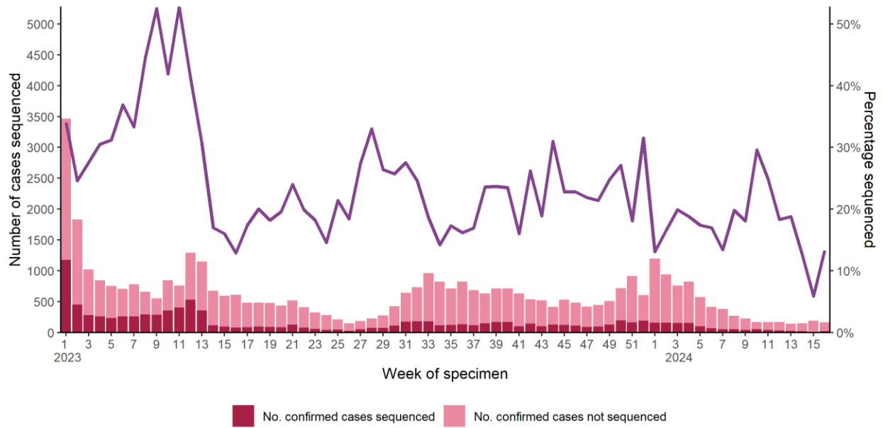
Figure 2: Number of confirmed cases of COVID-19 notified, by number sequenced/not sequenced, and percentage sequenced, week 1 2023 to week 16 2024, Ireland.
