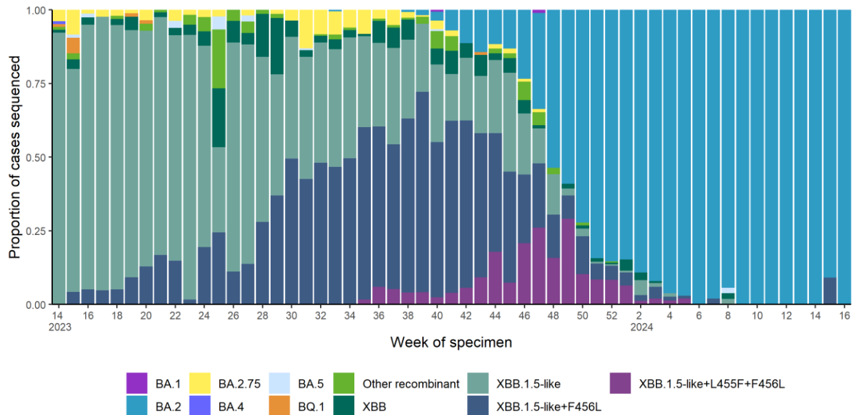
Figure 3b: Proportion of sequenced SARS-CoV-2 specimens by variant, specimen collection dates from week 14 2023 to week 16 2024, Ireland.
