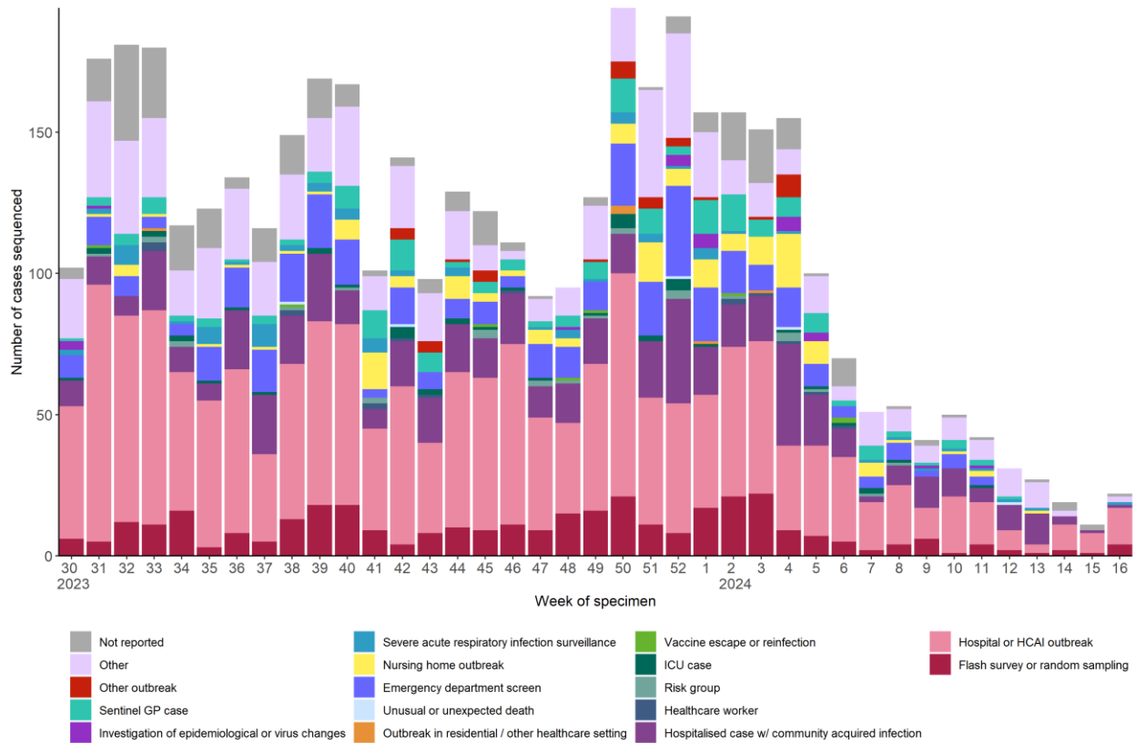
Figure 5: Reason for COVID-19 sequencing results provided from week 30 2023 to week 16 2024, Ireland.
