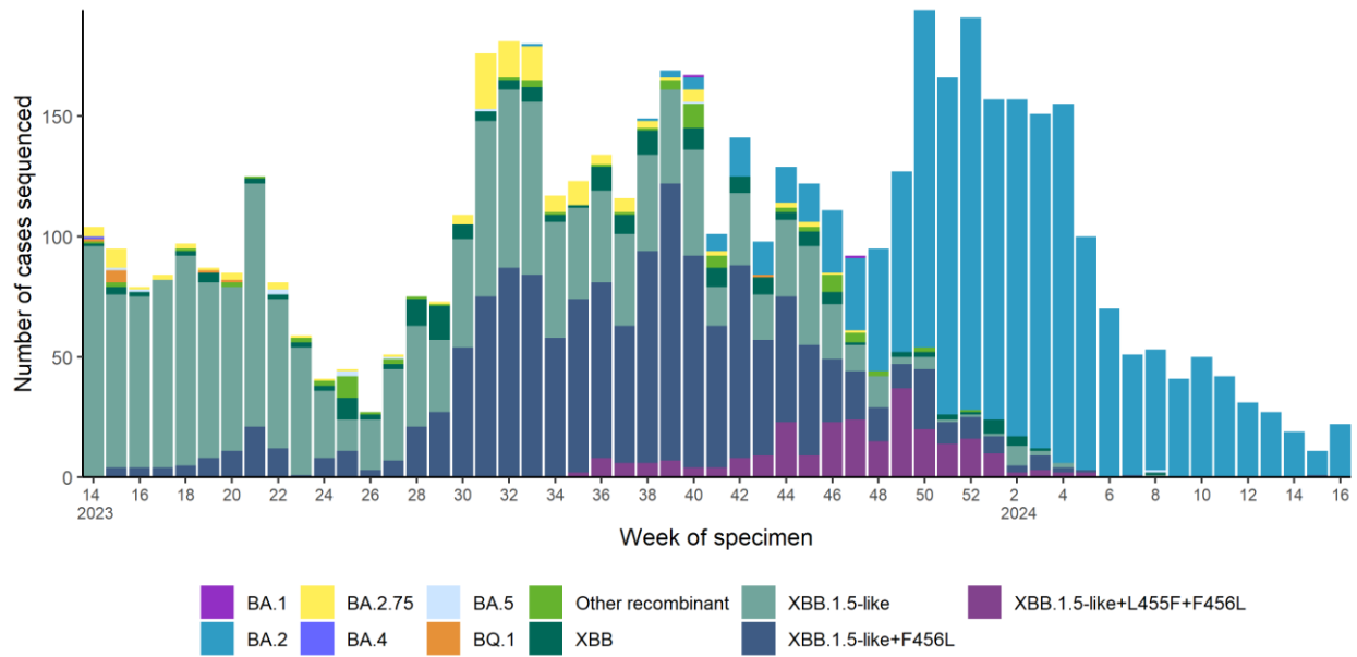
Figure 3a: SARS-CoV-2 whole genome sequencing results, specimen collection dates from week 14 2023 to week 16 2024, Ireland. 1
